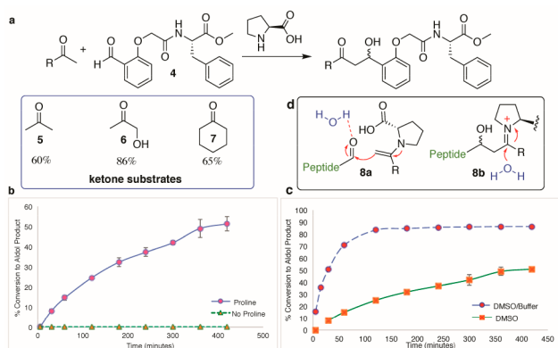
Figure 2. Model aldol bioconjugation between (a) phenylalanine aldehyde 4 and ketones ( 5–7 ) catalyzed by proline. (b) Comparison of uncatalyzed and proline-catalyzed (100 mM) reaction rates in DMSO at 37 °C between 4 (1 equiv., 7 mM) and hydroxyacetone 6 (12 equiv., 84 mM). (c) Comparison of reaction in 100% DMSO versus 1:1 sodium phosphate buffer (pH 7.4):DMSO. (d) Proposed role of water in increasing reaction kinetics.
