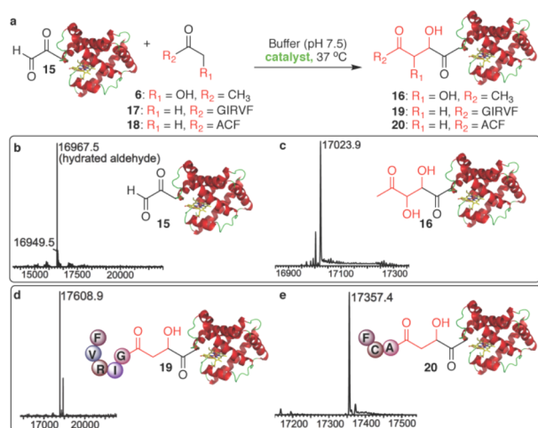
Figure 4. Organocatalyzed protein modification. (a) Ligation of N-terminal myoglobin aldehyde 15 (0.15 mM) with different ketones ( 6 , 17 , and 18 (10 mM)) using either proline (b, c) or O-tBu-Thr (d, e) (100 mM) as catalysts in 25 mM phosphate buffer (pH 7.5) and up to 15% DMSO at 37 °C. Deconvoluted ESI-MS spectra of (b) unreacted myoglobin aldehyde 15 , (c) myoglobin hydroxyacetone bioconjugate 16 generated by reaction with 6 , and (d and e) myoglobin-peptide bioconjugates 19 (60%) and 20 (40%) generated by reaction with peptide ketones GIRVF 17 and ACF 18 .
